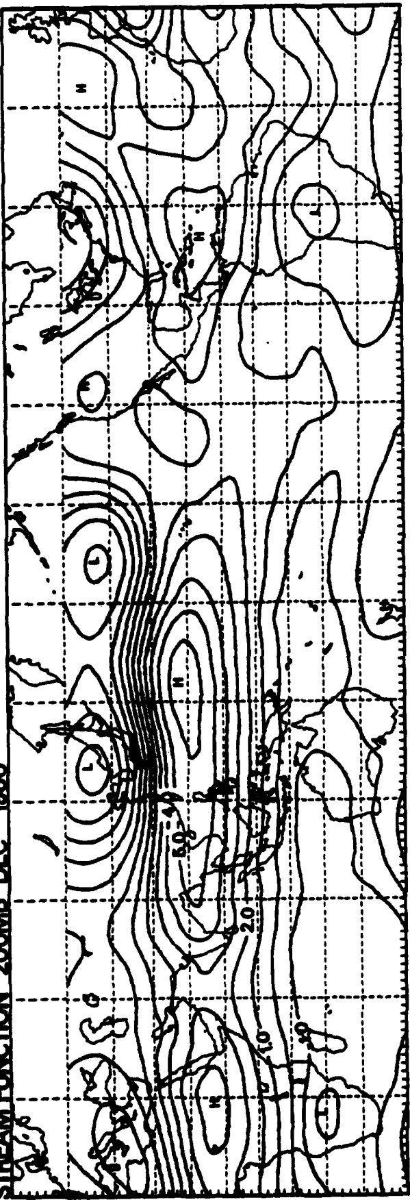
STREAM FUNCTION 200MB DEC 1980
